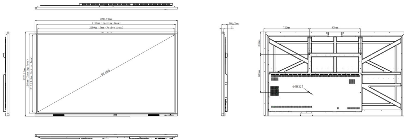
98": ST-98-CONNECT-PRO5
